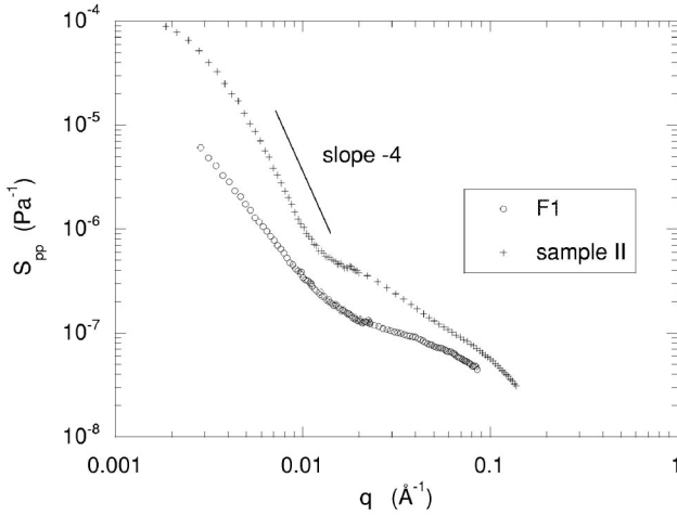
FIG. 6. Comparison between polymer structure factors S_{pp}(q) in sample F1 ( \circ ) and sample II ( + ). The region of Porod scattering in the latter case is indicated by a straight line with slope -4 .
